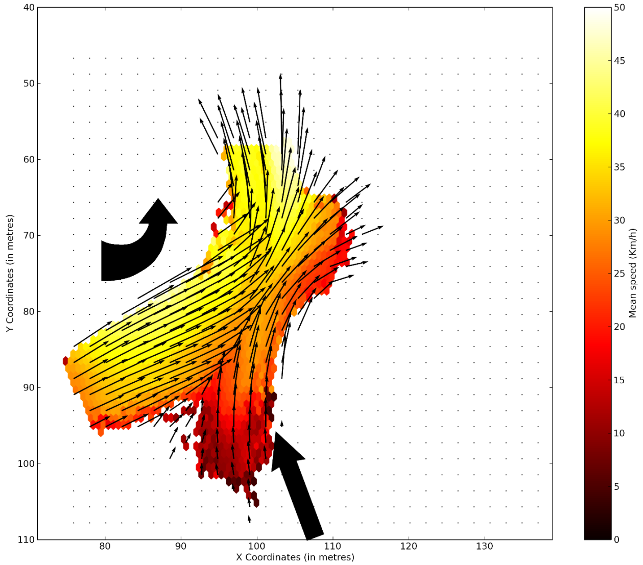
Figure 6 – Sample mean speed map (2-dimensional histogram of mean speed observations in a hexagonal grid) with overlaid velocity vector field (large black arrows indicate movements in the center and on the approach). Speeds inside the roundabout are noticeably faster than at the approach or exit.
