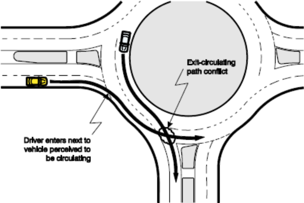
Figure 1 – Comparison of conflict points inside of a traditional intersection and a roundabout. Image source: NHCRP Report 672 (3).
